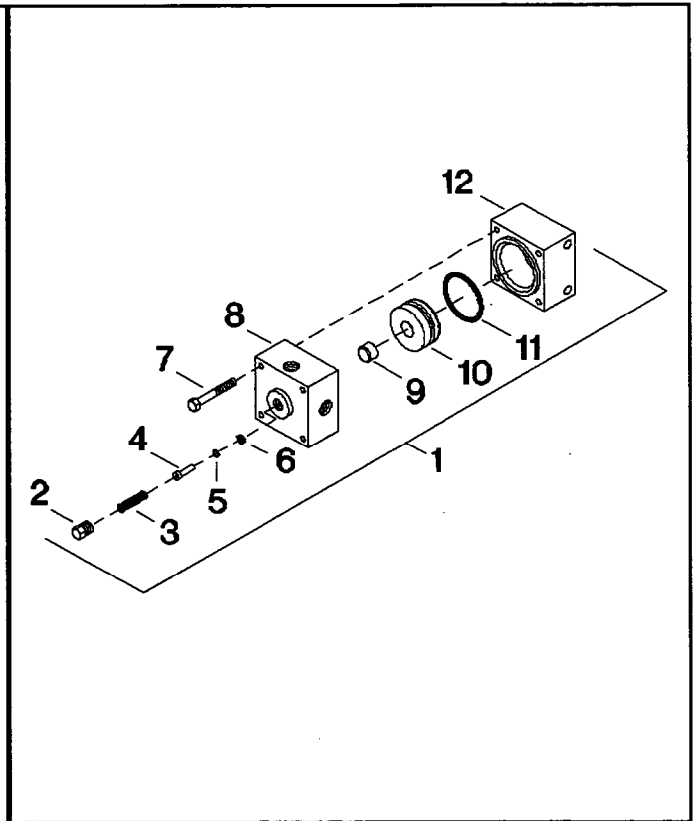
FIGURE 2. UL 104B VALVE
