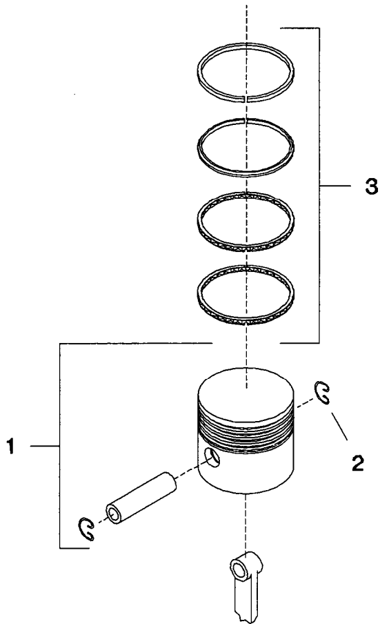
FIGURE 7. PISTON/PIN AND RING ASSEMBLY (5.5 INCH)
