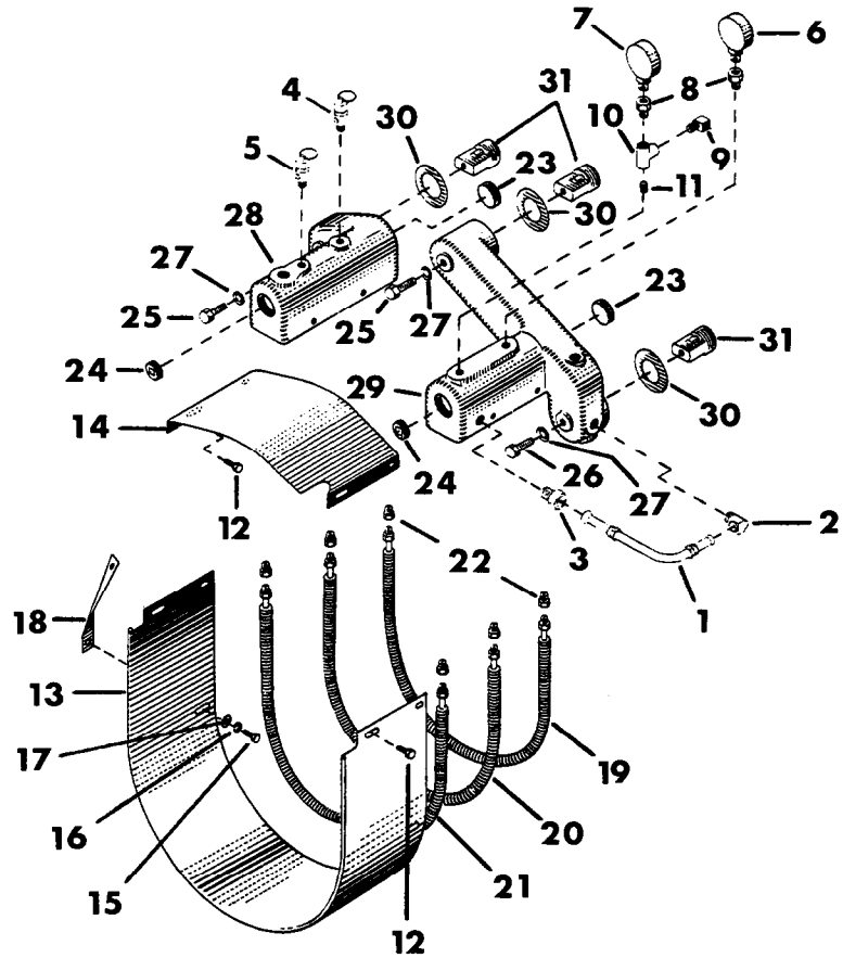
FIGURE 11. 15T2 INTERCOOLER ASSEMBLY.
