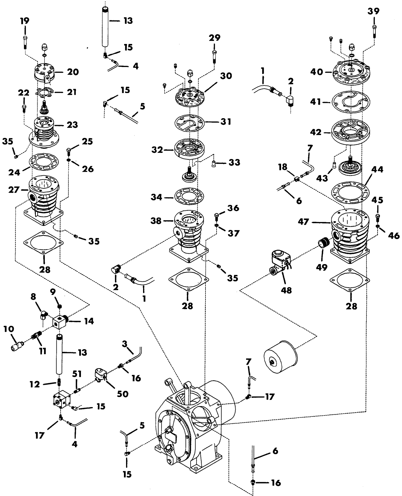
FIGURE 5. MODEL 15T2 BARE COMPRESSOR.
