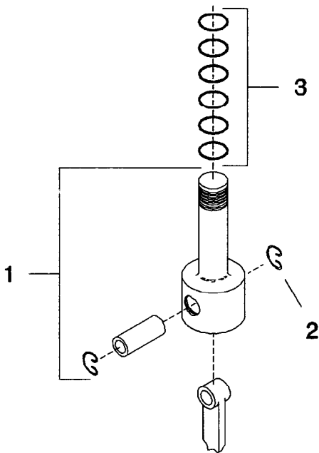
FIGURE 5. PISTON/PIN AND RING ASSEMBLY (1.625 INCH)
