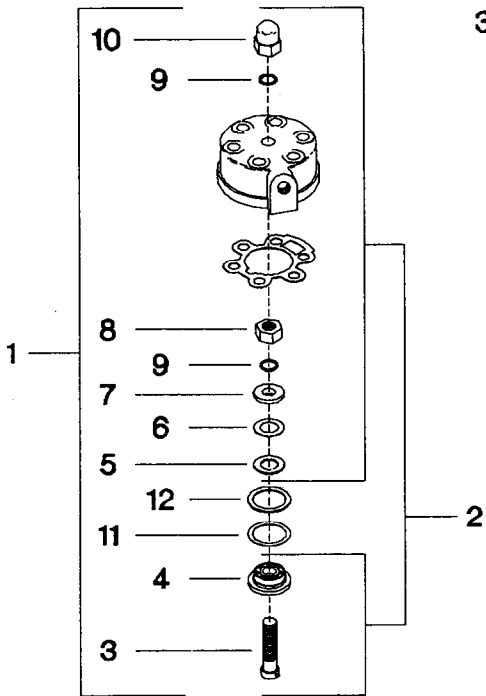
FIGURE 8. 20 GA. VALVE ASSEMBLY
