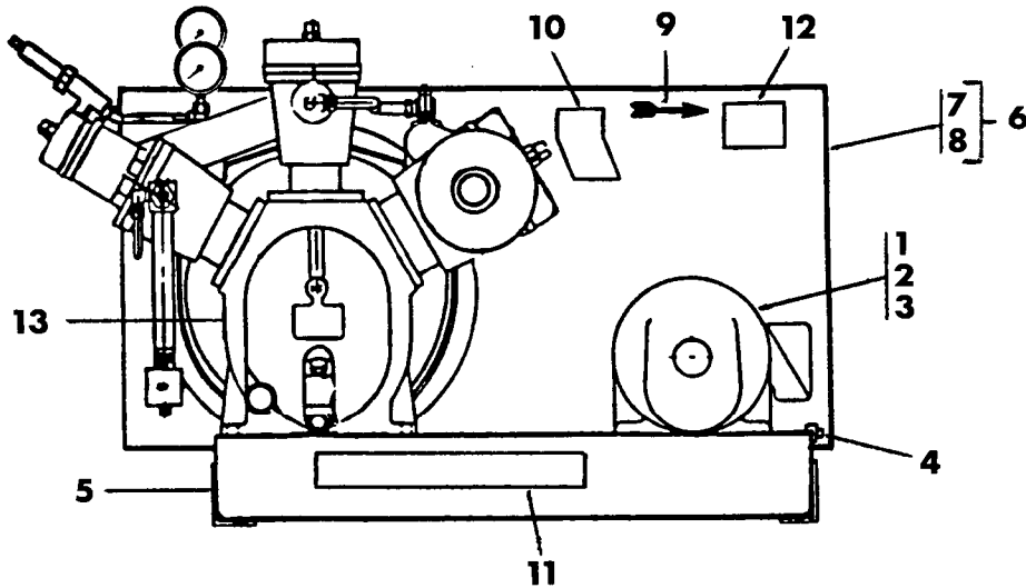
FIGURE 7. COMPRESSOR DRIVE, SUB-BASE, AND ACCESSORIES.
