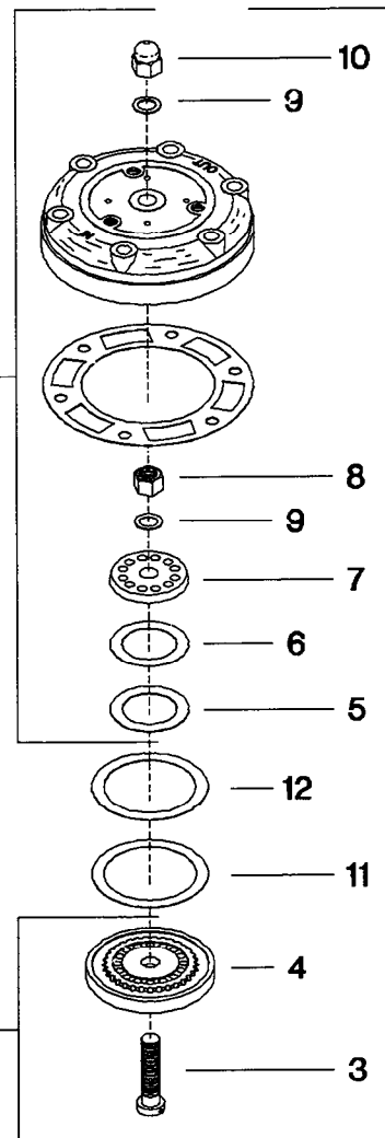
FIGURE 10. 55 GA. VALVE ASSEMBLY
