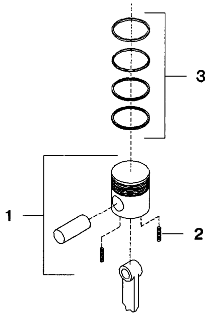
FIGURE 6. PISTON/PIN AND RING ASSEMBLY (3 INCH)
