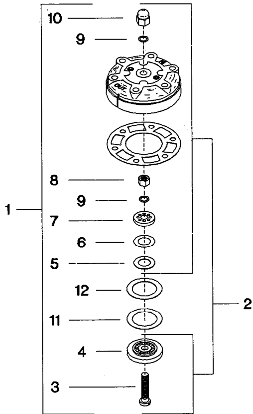
FIGURE 9. 35 GA. VALVE ASSEMBLY
