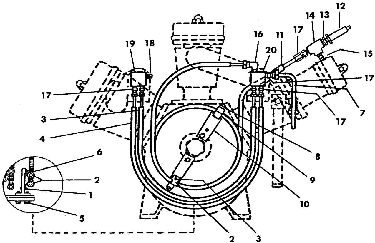
FIGURE 12. 15T2 AFTERCOOLER ASSEMBLY.
